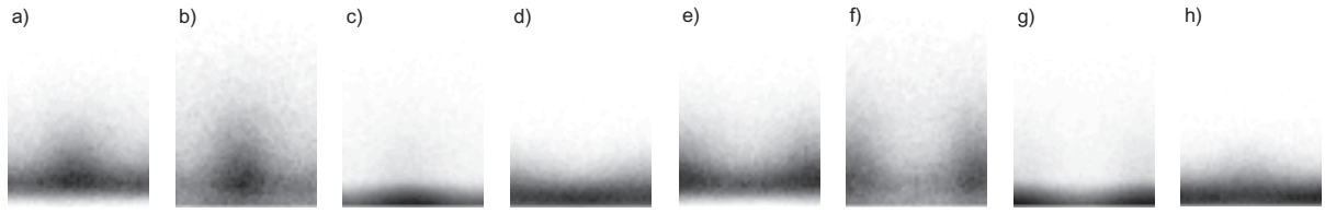
Figure 3. Density field obtained by phase- and space-averaging particle positions from the MD simulation. One single wavelength is shown along eight equidistant phases (a)–(h).
